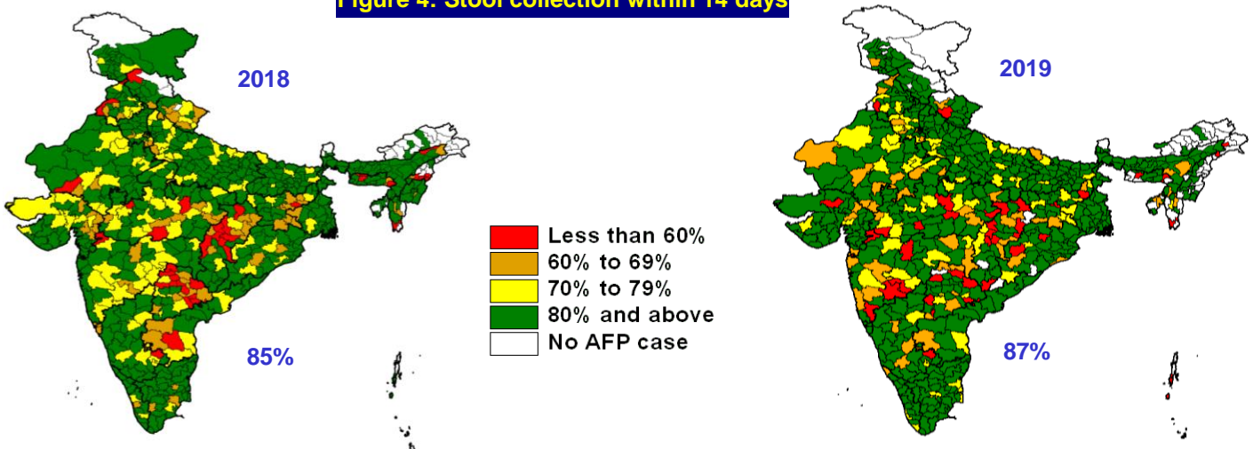
Figure 4: Stool collection within 14 days
